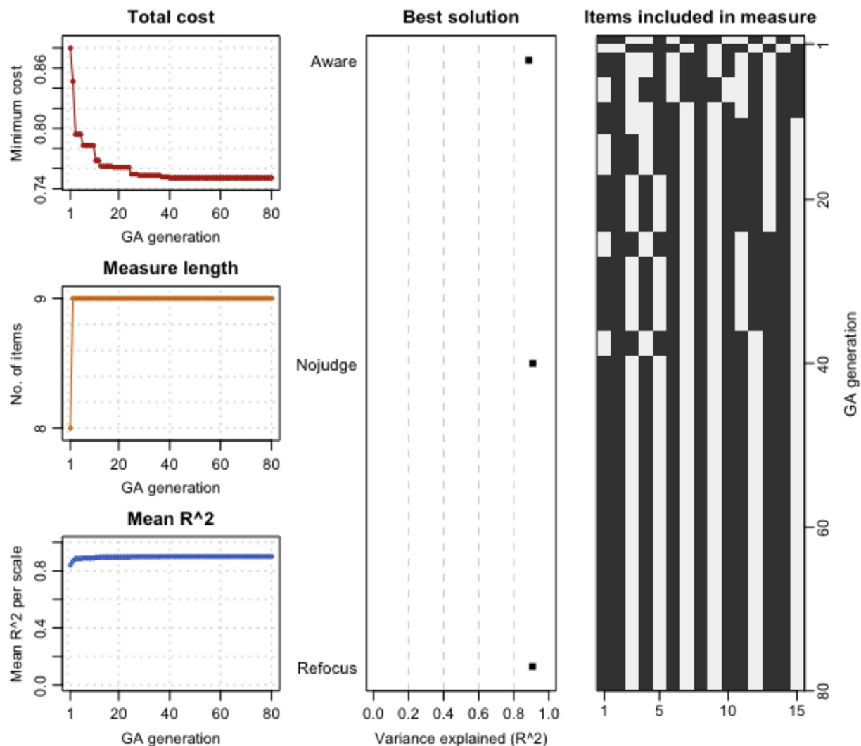
Fig. 1. Plots demonstrating output from example genetic algorithm run. The left three plots display improvements across generations for: cost of shortening measure (top), measure length (middle), and variance explained by short measure (bottom). The central plot demonstrates the variance explained by the best solution for each subscale. The right hand plot shows the selected items (in black), with high variation in the first runs (top of plot) and a stable solution emerging after 40 generations (bottom half of plot).
