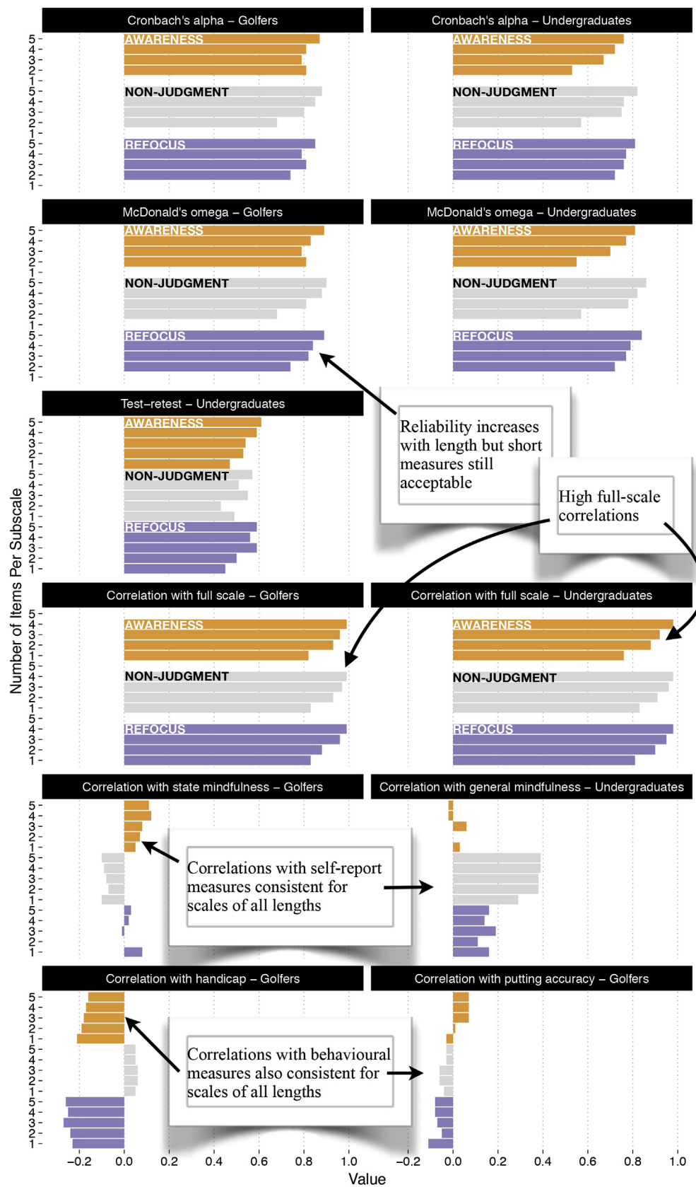
Fig. 2. Reliability and validity metrics for full measure (5-items per subscale) and shortened measures.
